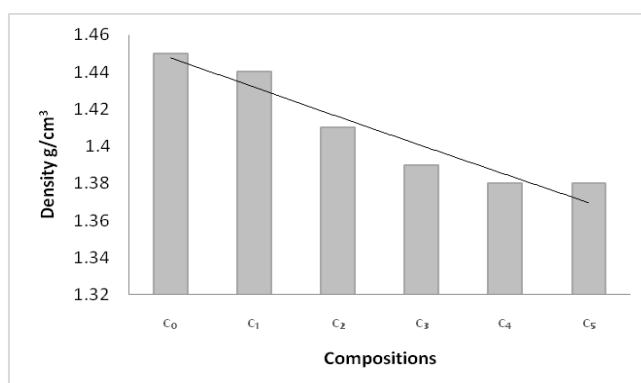
Fig. 3 Density variations as a function of percentage of (OPC)
