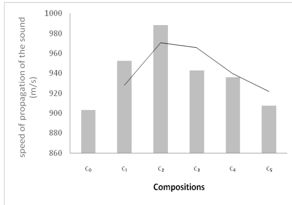
Fig. 6 Speed of propagation of the sound as a function of (OPC) dosage
