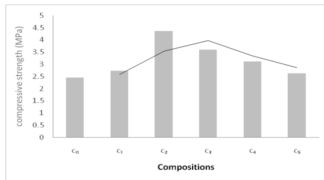
Fig. 5 Compressive strengths as a function of (OPC) dosage
