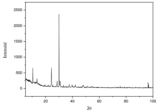
Fig. 2 The X-ray diffraction (XRD) of Temchemt
