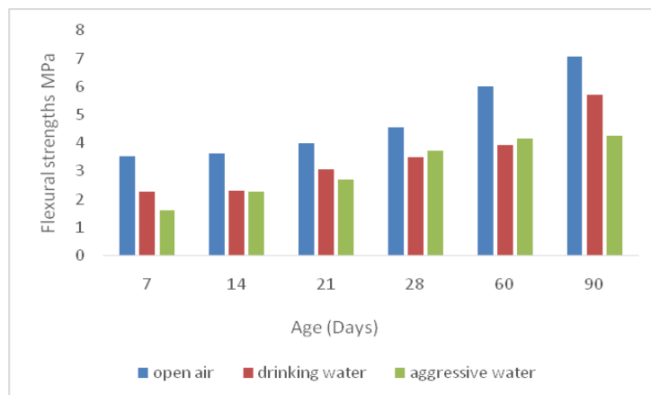
Fig. 12 Flexural strength as a function of time
