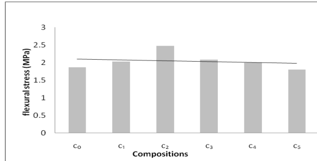
Fig. 4 Flexural strengths as a function of (OPC) dosage
