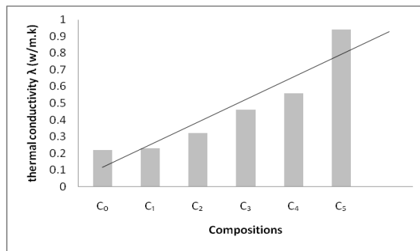
Fig. 7 Thermal conductivity of bricks as a function of the percentages of (OPC)
