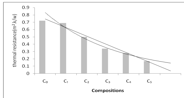
Fig. 8 Thermal resistance of bricks as a function of the percentages of (OPC)
