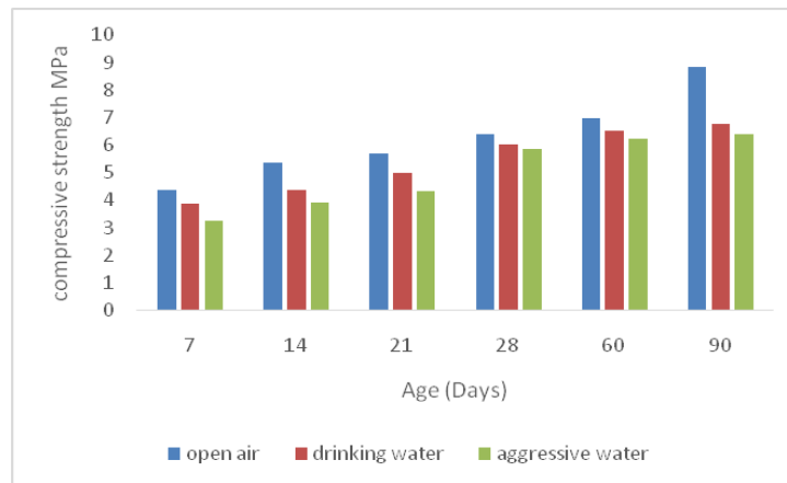
Fig. 13 Variations of the compressive strength of bricks as a function of time
