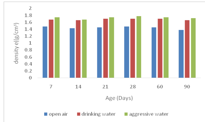
Fig. 11 Variations of brick density as a function of time
