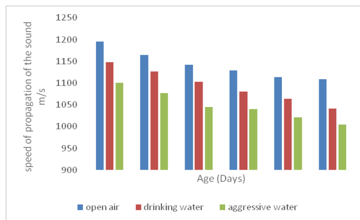
Fig. 14 Variations of sound speed as a function of time
