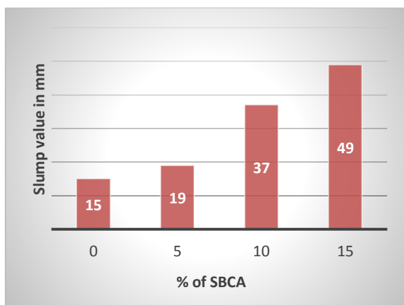
Fig. 2 Slump value vs. % of SCBA
