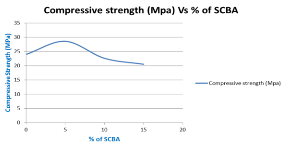
Fig. 4 Compressive strength for 28 days.
