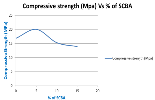
Fig. 3 Compressive strength for 7 days.
