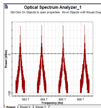
Fig. 12 Optical spectrum of VLC system
