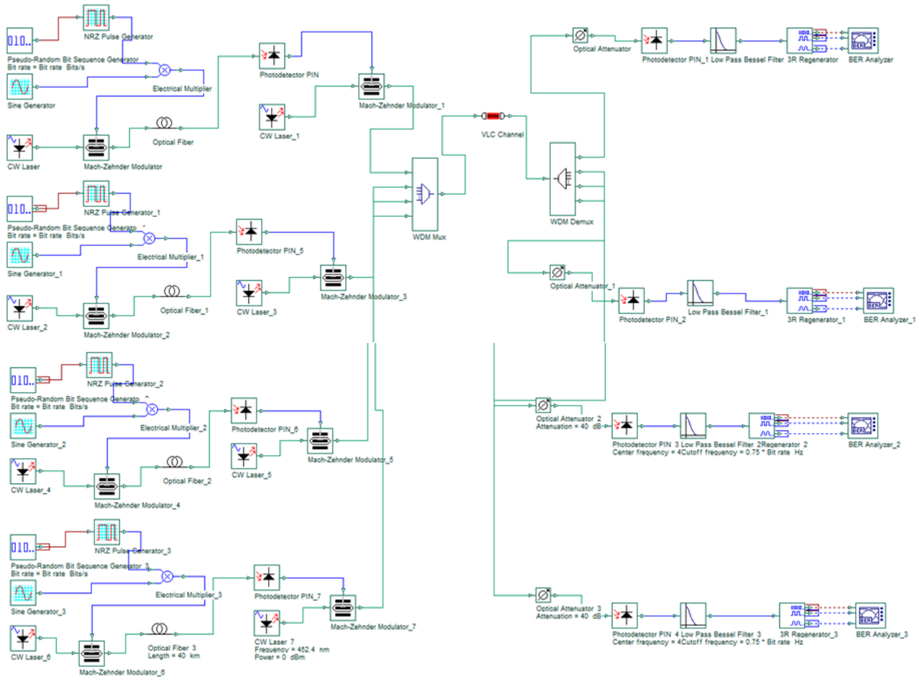
Fig. 2 Radio over fiber-VLC system based on WDM in optisystem
