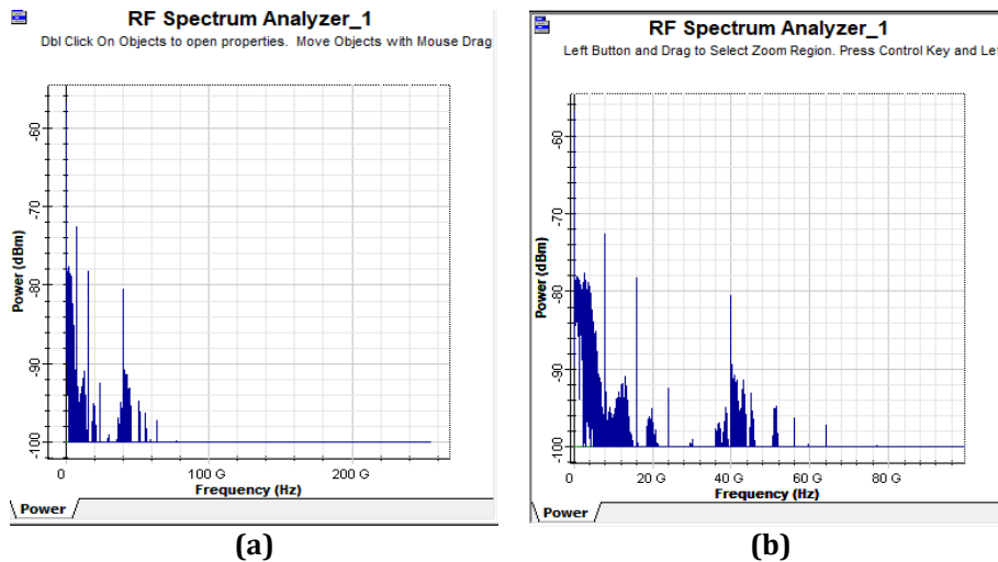
Fig. 8 RF spectrum for the RoF signals after photodetector PIN (a) Full spectrum; and (b) Close-in view of the showing the 40 GHz of Mmwave signal
