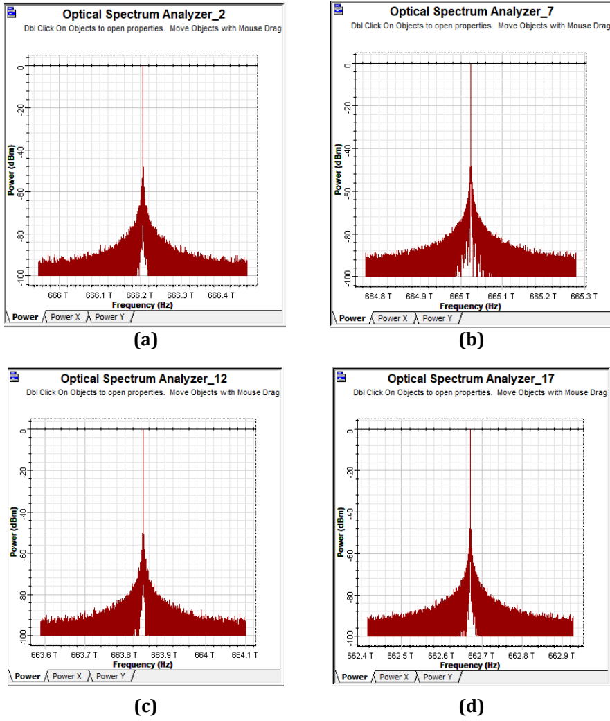
Fig. 9 The optical spectrum with CW laser is set at (a) 450 nm; (b) 450.8 nm; (c) 451.6 nm; and (d) 452.4 nm
