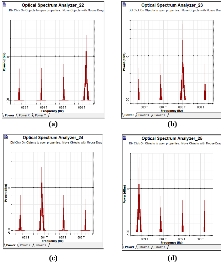
Fig. 13 Optical spectrum demultiplexed by WDM (a) 450 nm; (b) 450.8 nm; (c) 451.6 nm; and (d) 452.4 nm
