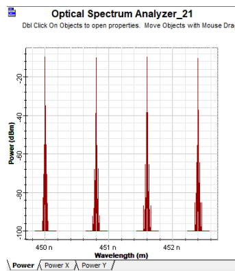
Fig. 11 Optical spectrum multiplexed by WDM
