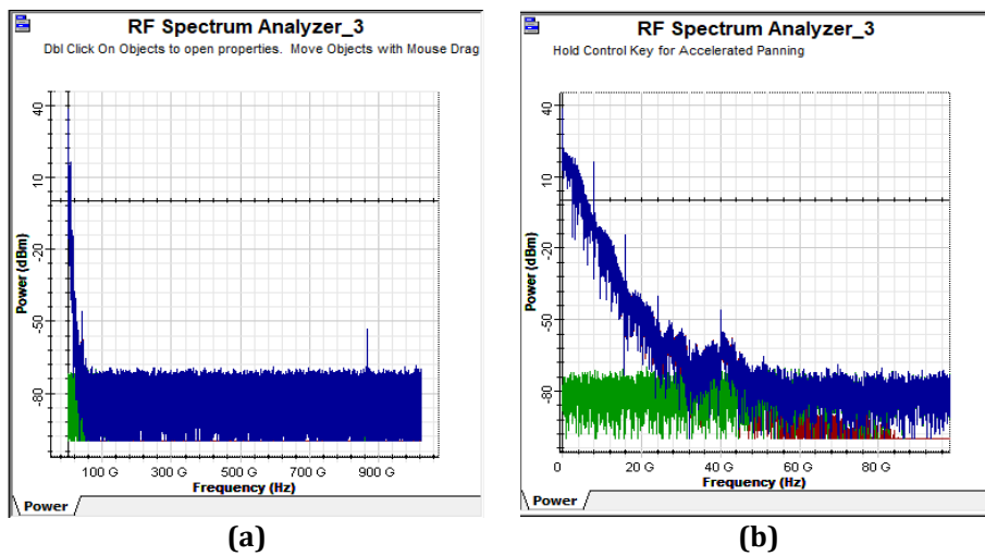
Fig. 14 RF spectrum for the RoF-VLC signal after PIN photodetector (a) Full spectrum; and (b) Close-in view of the showing the 40 GHz of Mmwave signal
