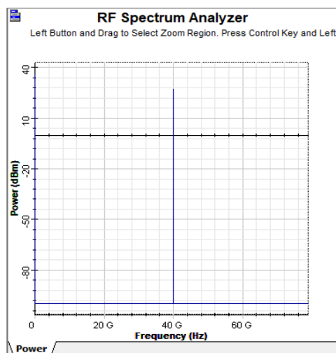
Fig. 4 The RF spectrum at the sine generator output showing the 40 GHz of mm-wave modulated data
