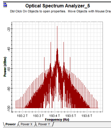
Fig. 7 Output of the fiber of 1550 nm
