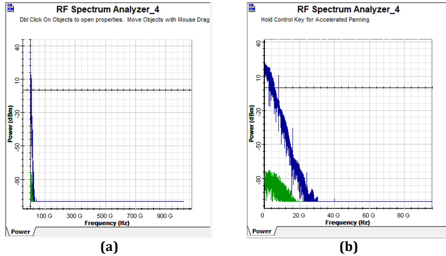
Fig. 15 Electrical spectrum for the RoF-VLC signals after Low pass Bessel filter (a) Full spectrum; and (b) Close-in view of the showing the 40 GHz of Mmwave signal
