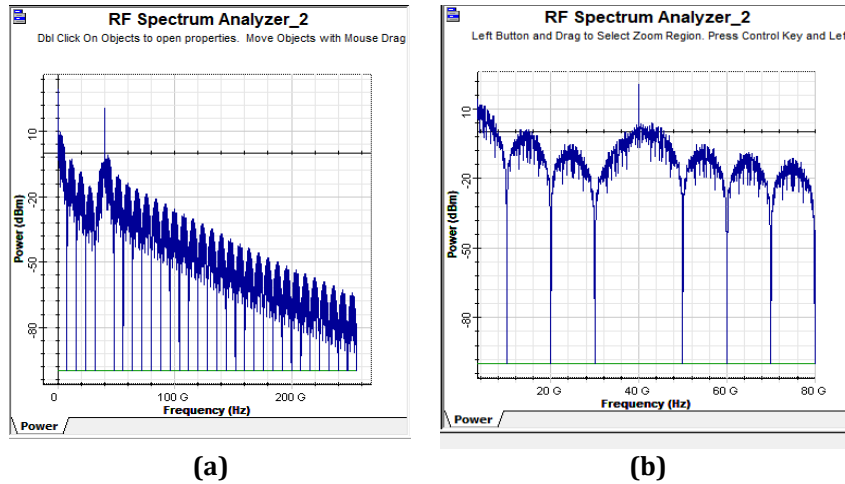
Fig. 5 The RF spectrum at the Electrical multiplier output (a) Full spectrum; and (b) Close-in view of the upper sideband showing the 40 GHz of mm-wave signal mix with 8 Gbps of NRZ
