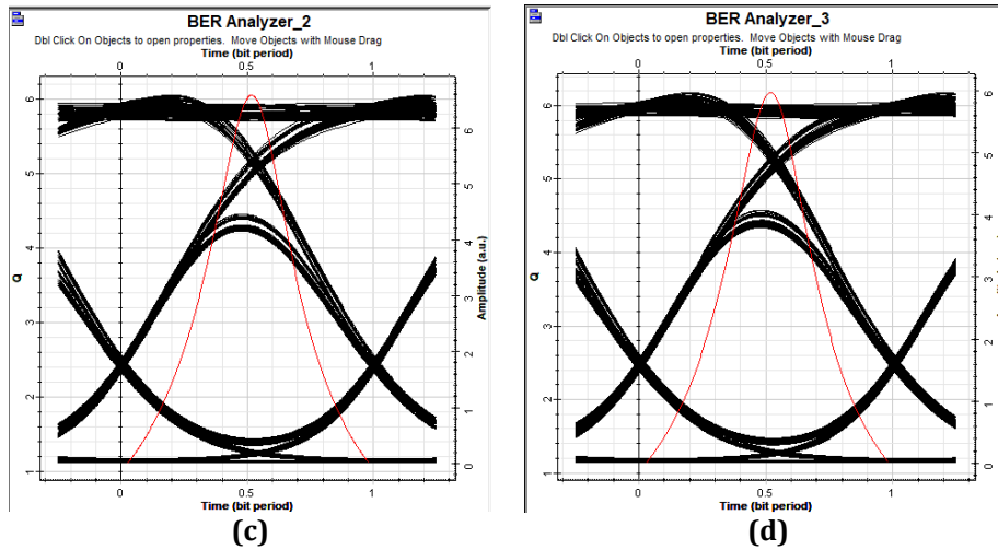
Fig. 16 The eye diagram for radio over fiber-VLC system based on WDM. (a) Eye diagram at channel 1; (b) Eye diagram at channel 2; (c) Eye diagram at channel 3; and (d) Eye diagram at channel 4
