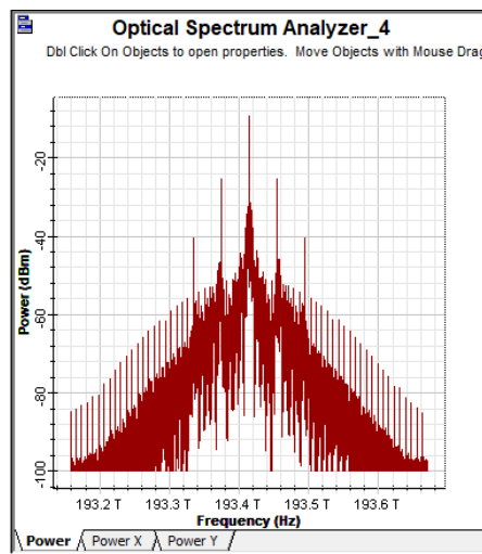
Fig. 6 Output of the MZM which is from CW laser of 1550 nm
