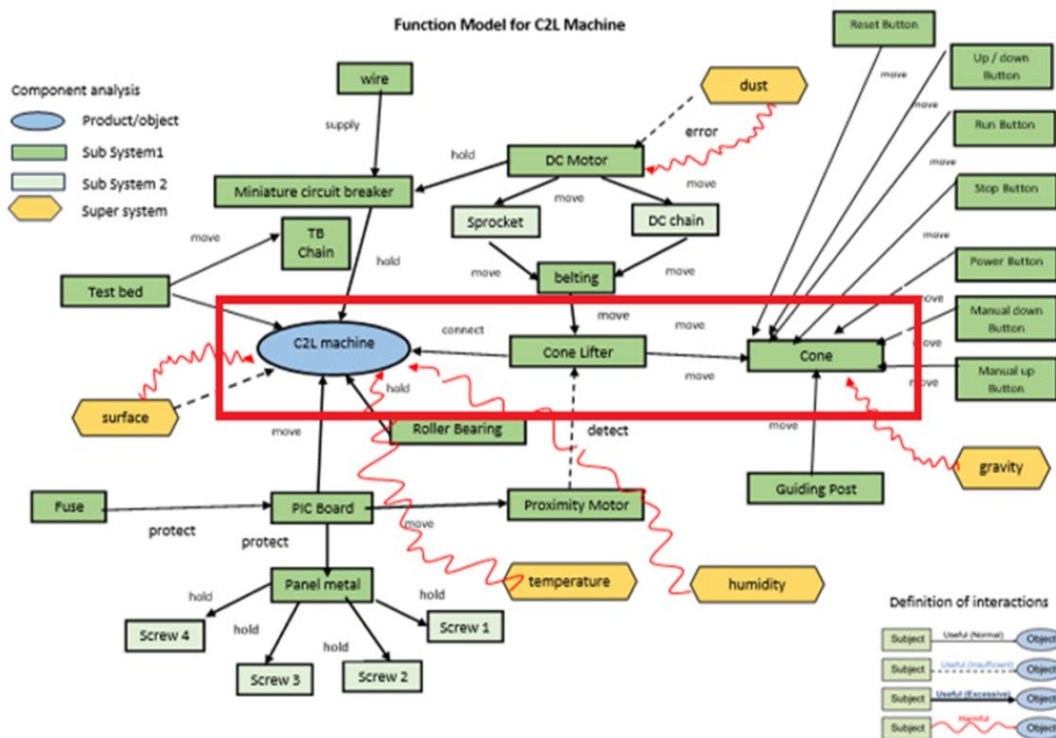
Fig. 5 The function analysis model (FAM) of C2L machine
