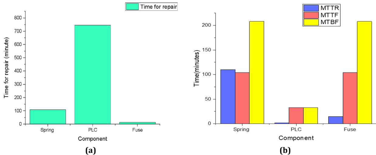
Fig. 7 The reliability experiment of C2L (a) The Graph of test motion B; (b) The graph of reliability for test motion B
