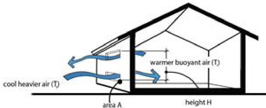
Fig. 12 - Stack Effect ventilation
