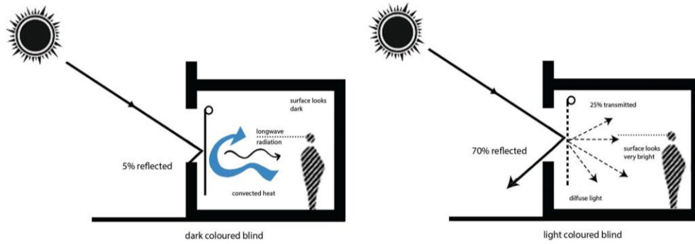
Fig. 6 - Performance of various blind materials
