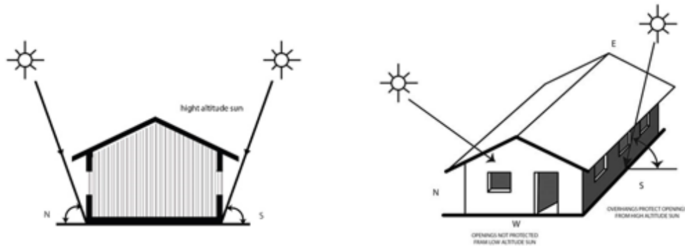
Fig. 7 - Orientation of the east and west of building to provide shading to openings in long walls
