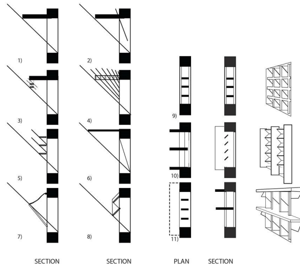
Fig. 9 - Various geometric shading devices
