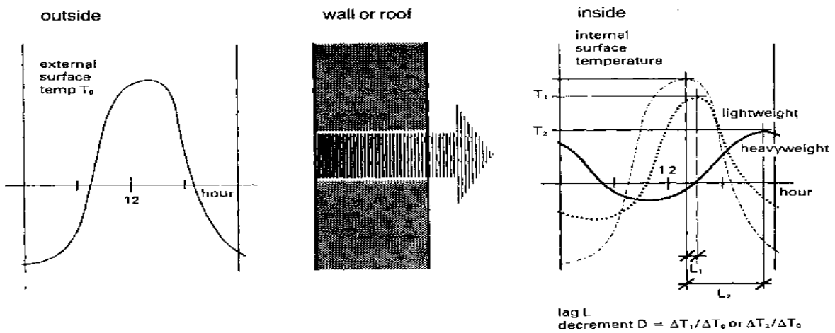
Fig. 4 - Time lag and decrement for heavy and light constructions
