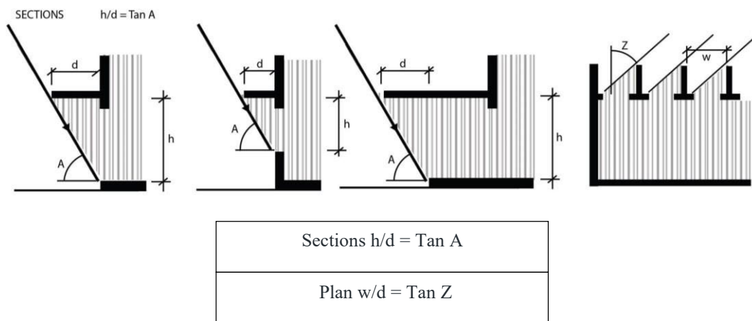
Fig. 8 - The Geometry of shading by overhangs
