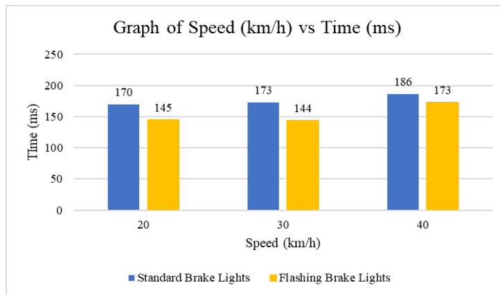
Fig. 10 - Average brake response time for both brake lights
