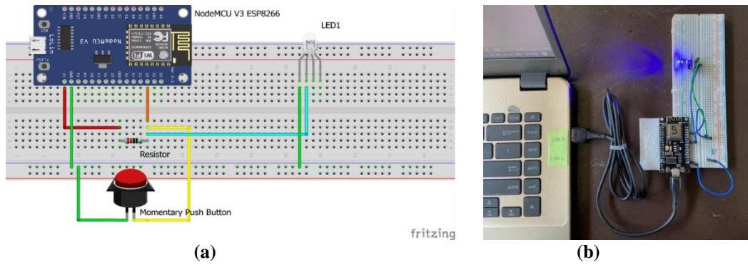
Fig. 2 - Server ESP8266 component setup; (a) Circuit Diagram, (b) Actual Hardware
