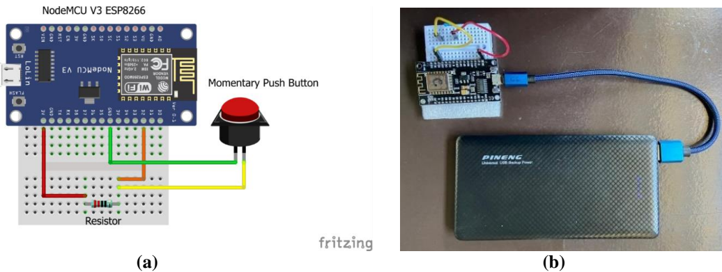
Fig. 3 - Client ESP8266 component setup; (a) Circuit diagram; (b) Actual Hardware
