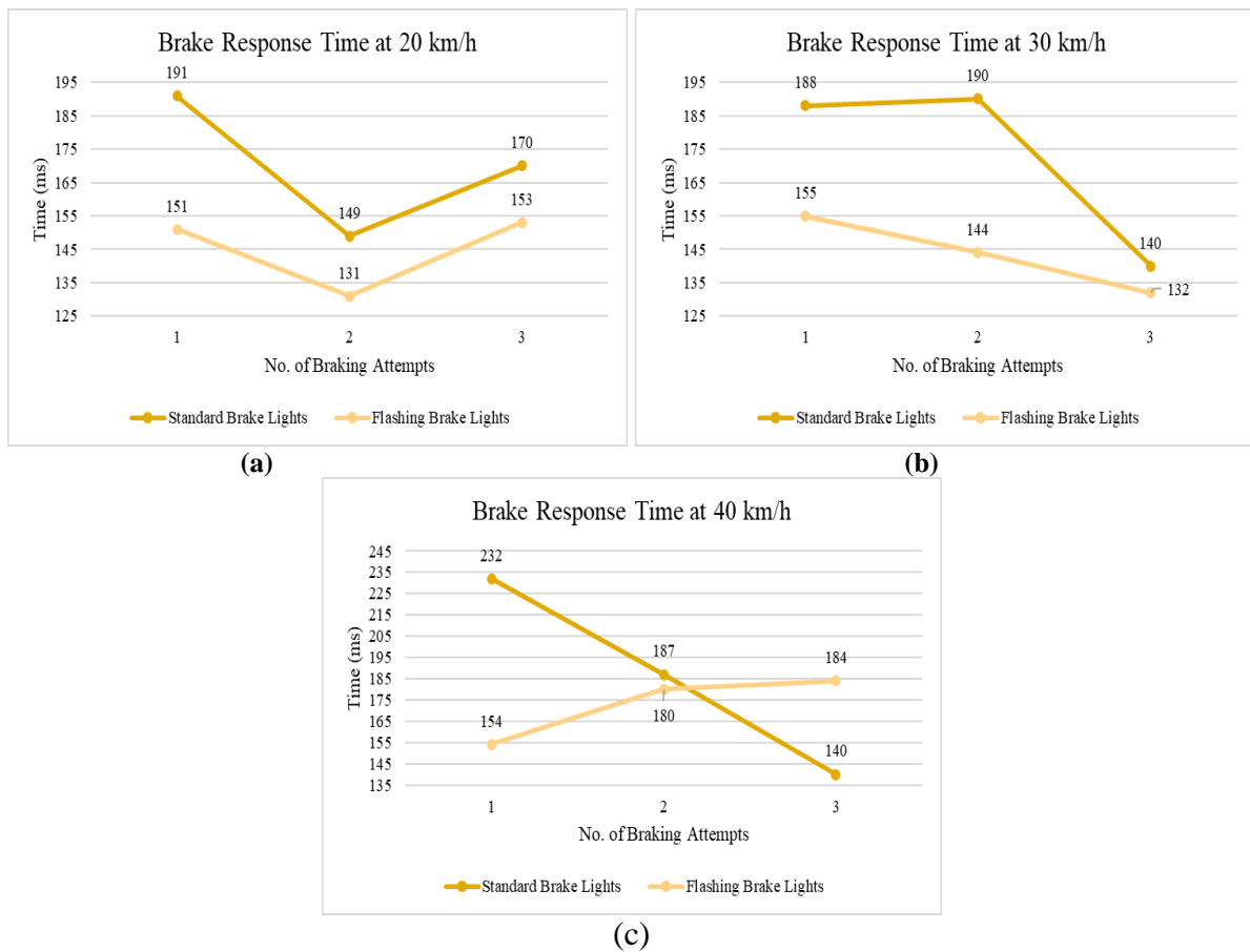
Fig. 9 - Brake response time for standard and flashing brake lights with three braking attempts; (a) At 20 km/h (b) At 30 km/h (c) At 40 km/h
