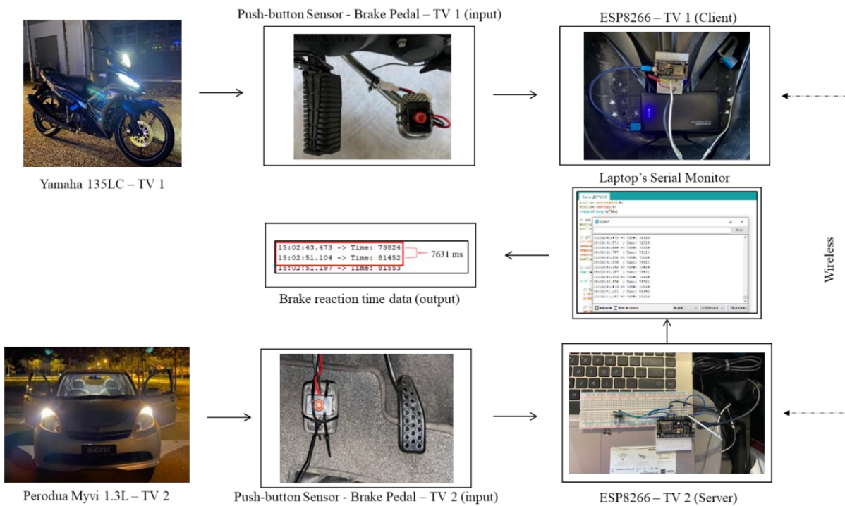
Fig. 5 - Overview of experiment setup
