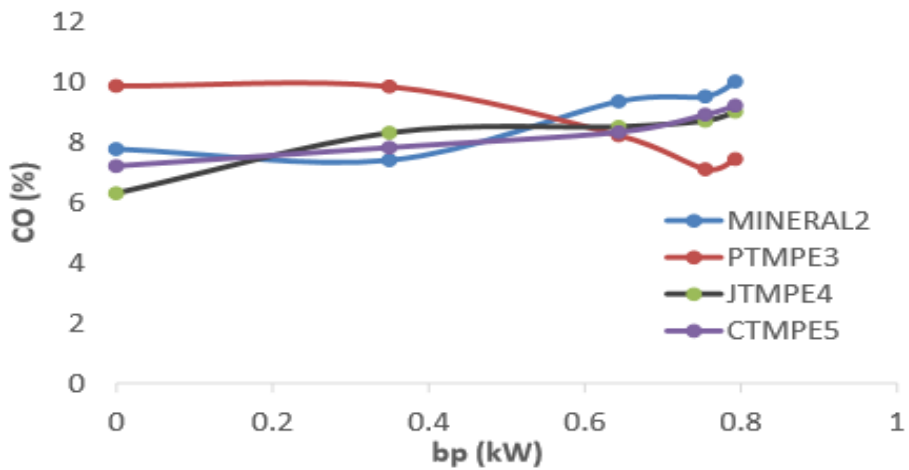
Fig. 4 - Exhaust emission (CO) versus power [25]
