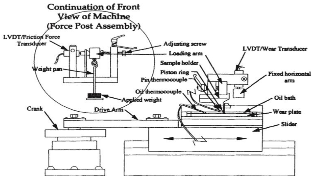
Fig. 1 - Schematic diagram of the testing machine [21]
