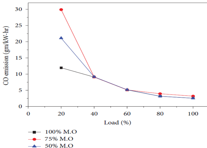
Fig. 9 - Comparison of CO emission under different load [27]
