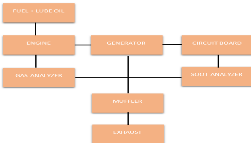
Fig. 2 - General arrangement of the experimental setup [21]
