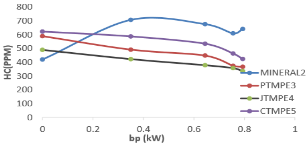
Fig. 5 - Exhaust emission (HC) versus power [25]
