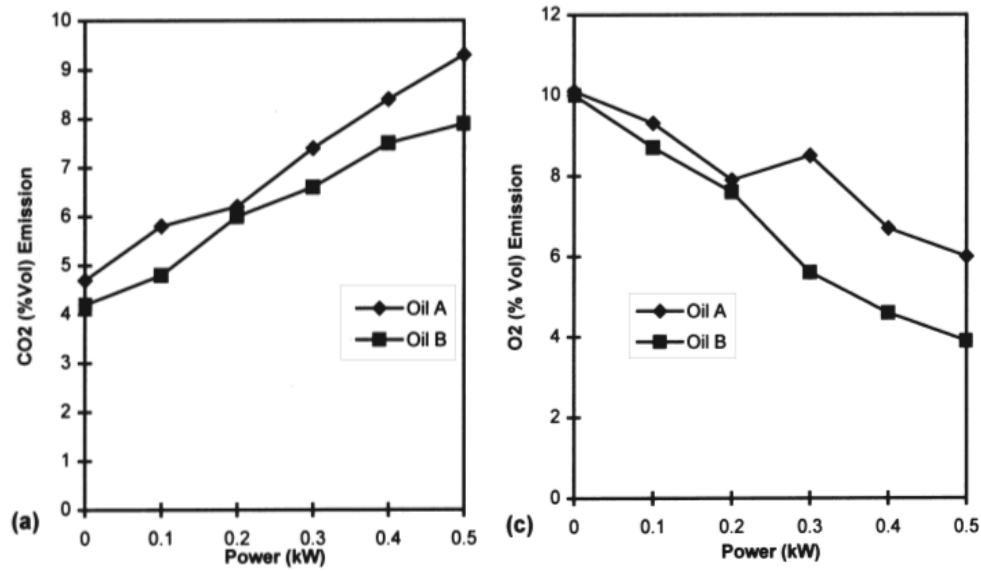
Fig. 3 - Exhaust emissions versus power (a) CO 2 ; (b) O 2 [21]
