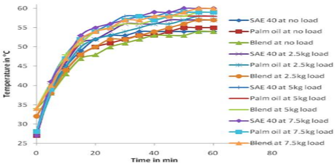
Fig. 7 - Coolant temperature versus time [24]
