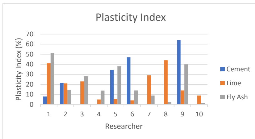
Figure 2: The graph for Researcher versus Plasticity Index (%)
