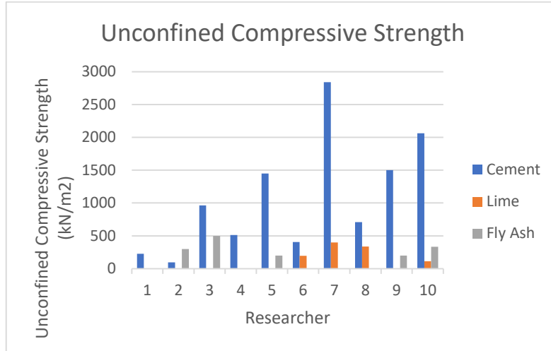
Figure 3: The graph for Researcher versus Unconfined Compressive Strength (kN/m²)
